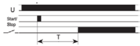
FZ39: Symmetrical recycling, ON start with Start/Stop pushbutton
