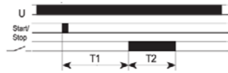
FZ70: Signal OFF delay
