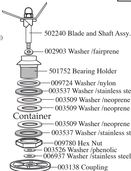
501832 Blending Assy.
