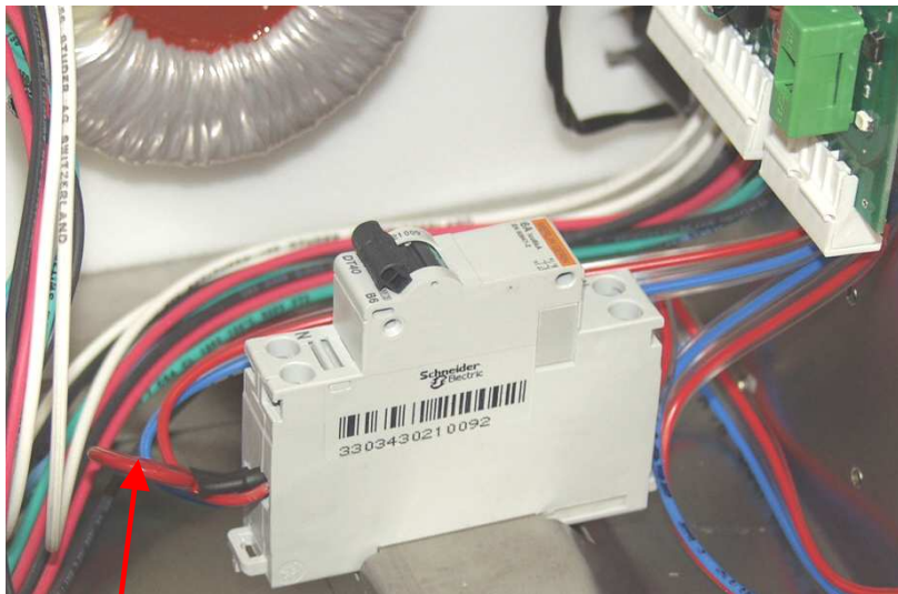
Varistor: 895401-85
