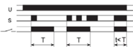
FZ07: Signal OFF pulse
