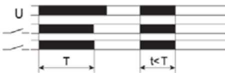
FZ19: ON pulse (1 timed contact + 1 instantaneous contact)
