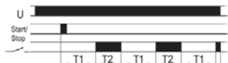
FZ40: Symmetrical recycling, OFF start with Start/Stop pushbutton
