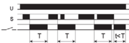
FZ08: Fixed pulse (0.5s) delayed
