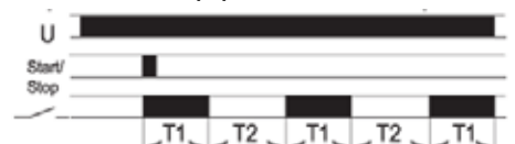
FZ39: Symmetrical recycling, ON start with Start/Stop pushbutton
