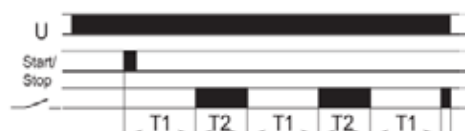
FZ40: Symmetrical recycling, OFF start with Start/Stop pushbutton
